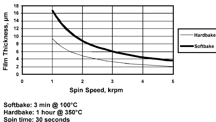
Figure 3.16. Spin speed vs thickness for photosensitive polyimide, Durimide* 7505 (low viscosity). (Courtesy Arch Chemicals, Inc.)
