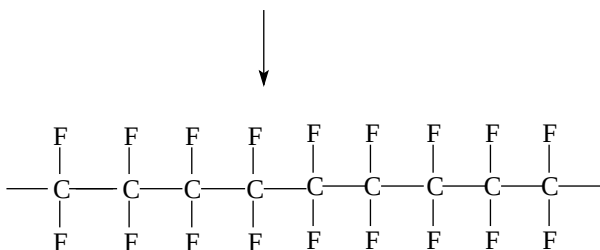
Figure 2.67. Polymerization reactions for fluorocarbon polymers.
