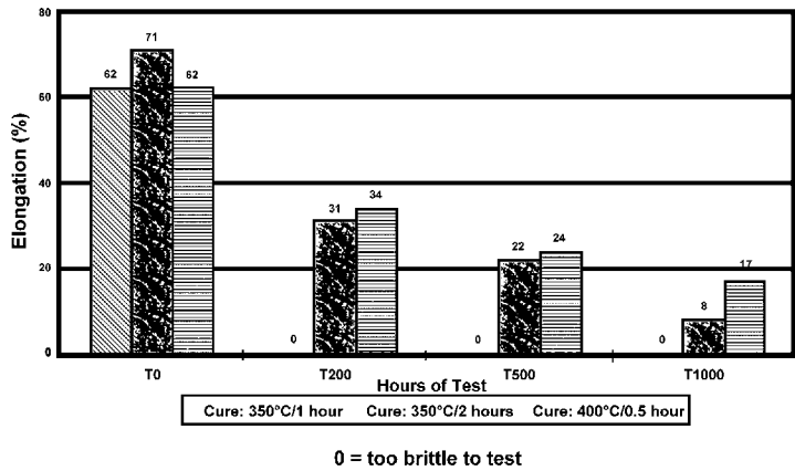
Figure 4.5. Effect of PCT conditions on the mechanical properties of Durimide® 7000 polyimide film. (Courtesy Arch Chemicals, Inc.)
