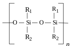
Figure 2.33. General structure for a linear silicone polymer.
