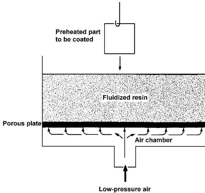
Figure 3.12. Fluidized-bed coating.
