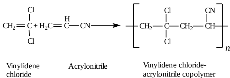
Figure 2.6. Vinyl-copolymer reaction.
