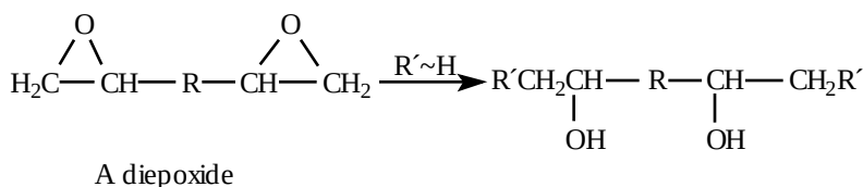
Figure 2.8. Epoxy chemistry.
